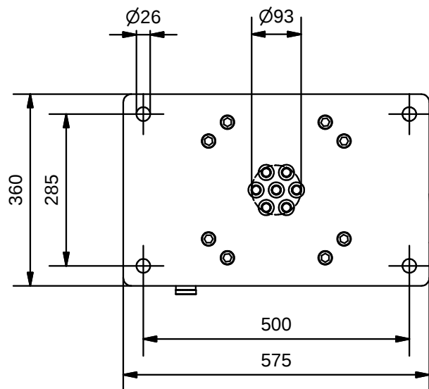
Bottom view (1:10)
